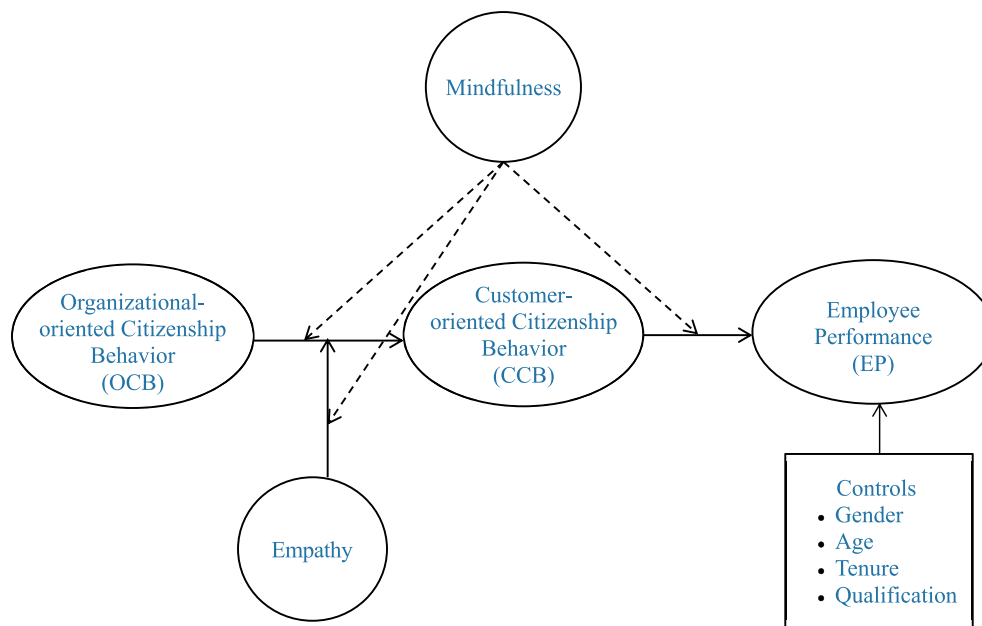
Fig. 1. Conceptual model.
